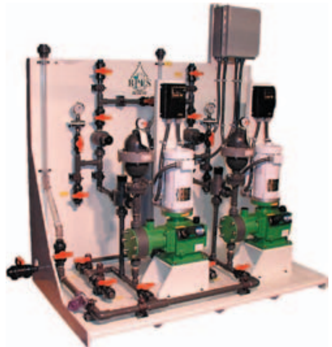
MS2 system designed for sodium hypochlorite in SCH-80 PVC shown with KM-254 metering pumps and stand alone local SCR controllers.
